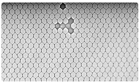
蜂窝检测
